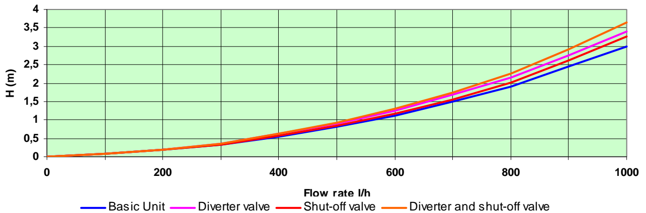
Primary circuit pressure loss
